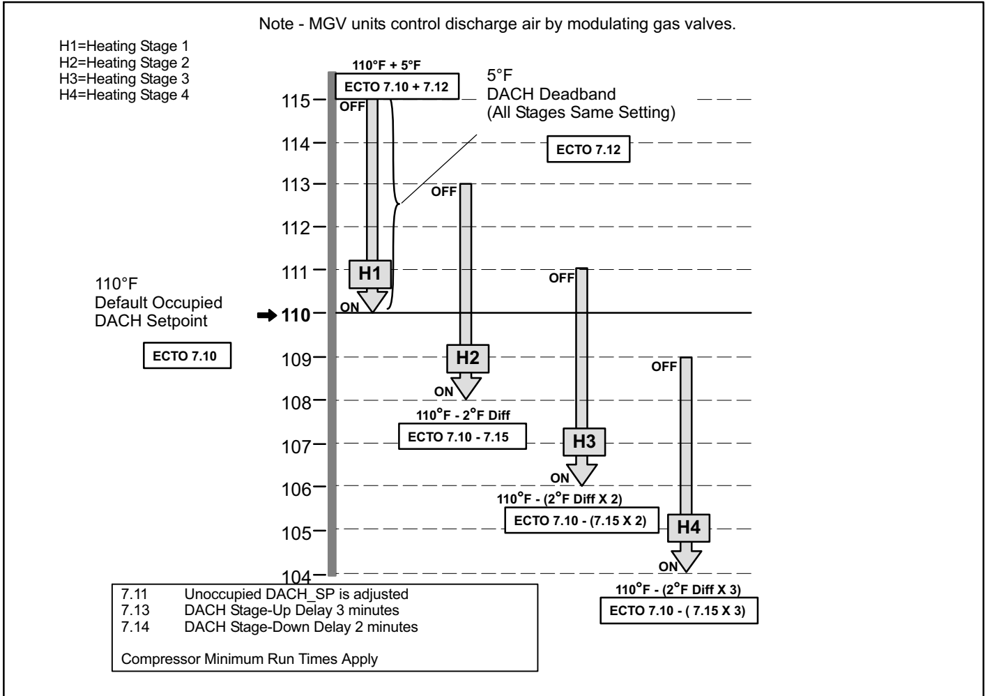
Figure 29. Discharge Air Control Heating (DACH) Stages - Default Values Shown
