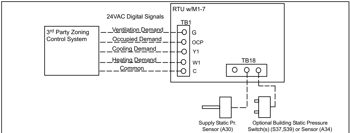
Figure 64. Field Wiring Summary for VAV Unit with Supply Air VFD
