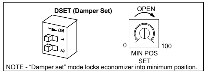
Figure 45. A56 EM1 Manual Damper Set DIP Switch
