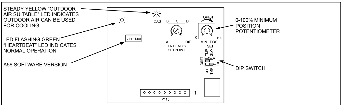
Figure 35. A56 (EM1) Economizer Board
