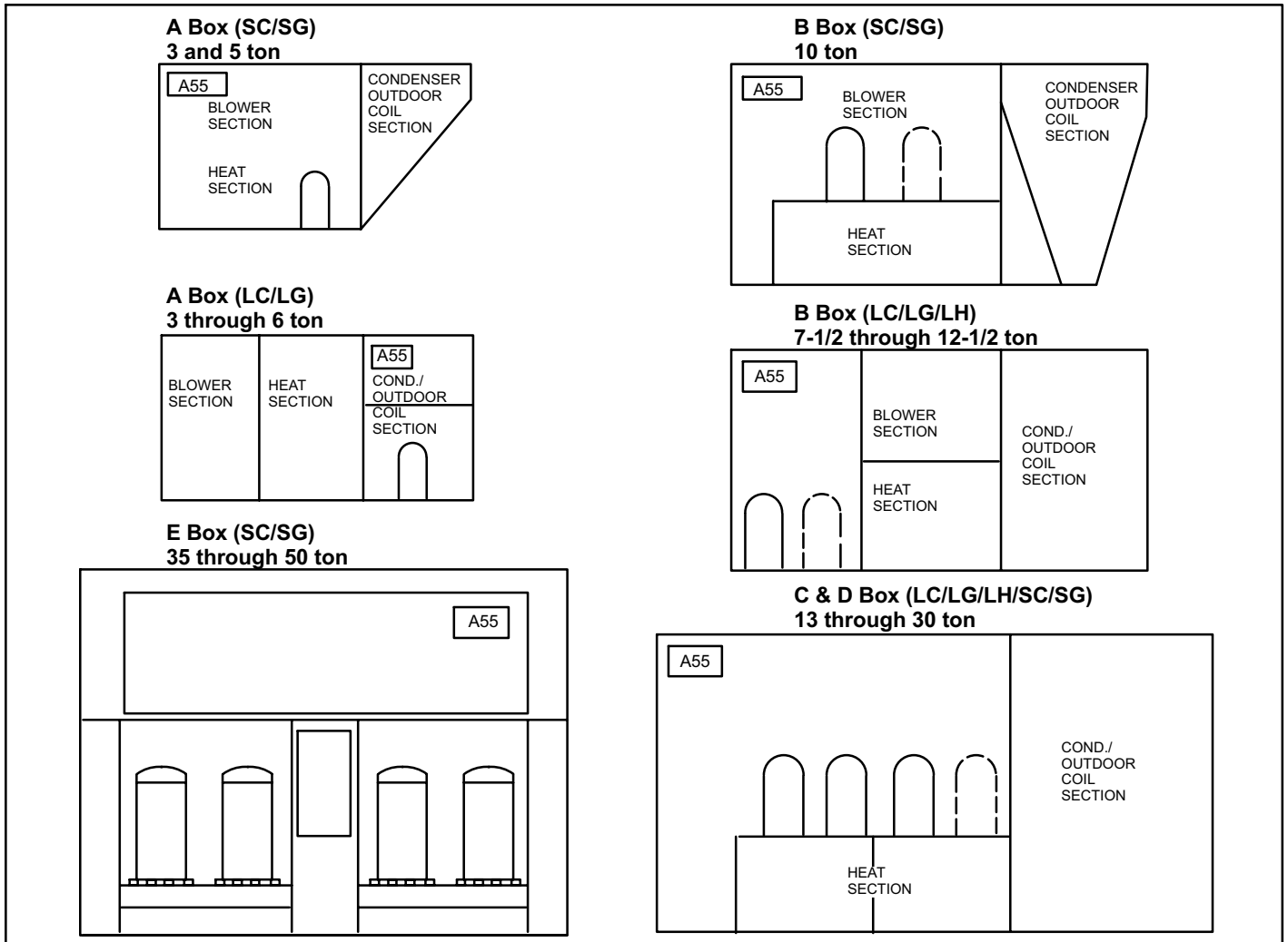
Figure 1. A55 (M1) Main Control Panel Location by Unit
