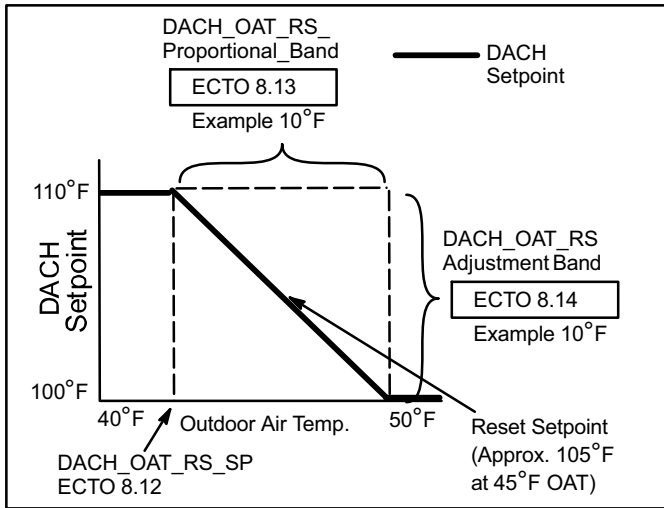
Figure 30. Outdoor Air Reset Example
