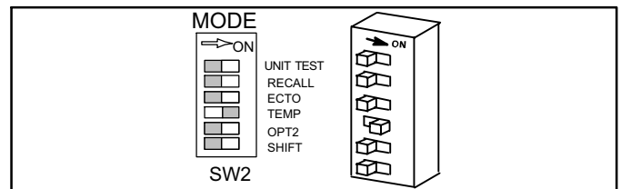
Figure 46. Display Sensor Input DIP Switch Setting
