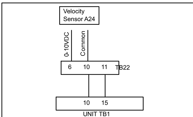
Figure 44. OAC Sensor Wiring
