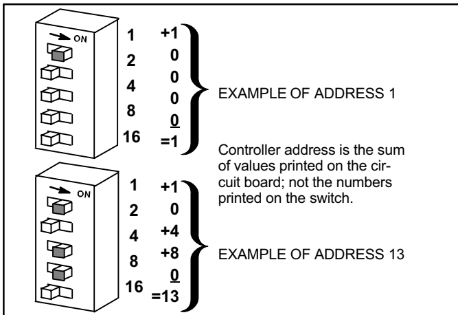
Figure 12. Address DIP Switch
