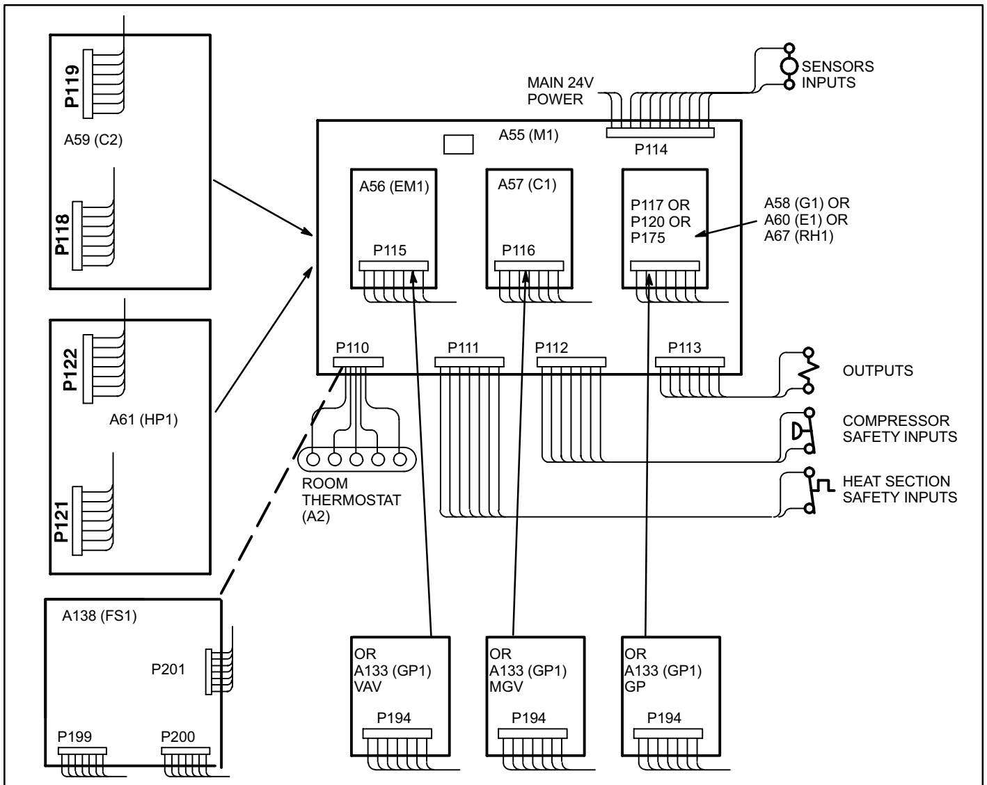
Figure 72. IMC Board Inputs and Outputs
