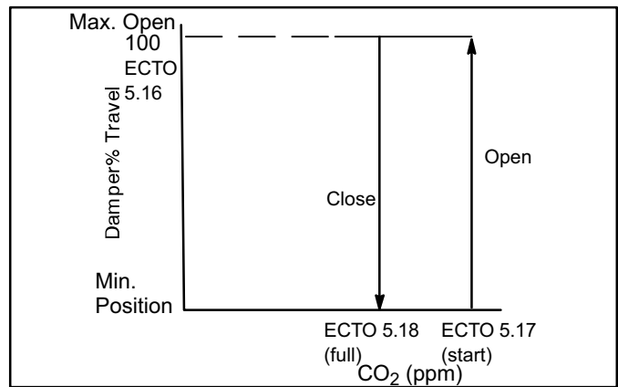
Figure 43. Setpoint Control IAQ Option
