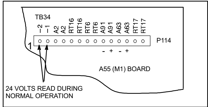
Figure 3. Check 24 Volt Supply To A55 (M1-7) Main Control Board
