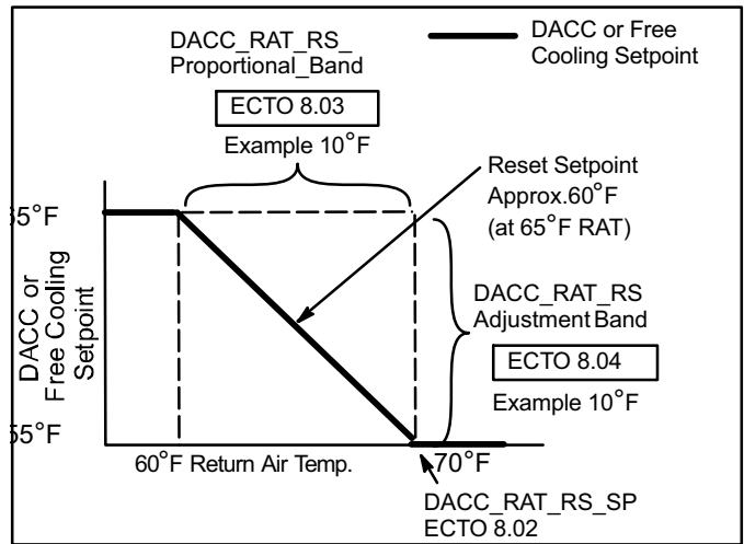
Figure 28. Return Air Reset Example
