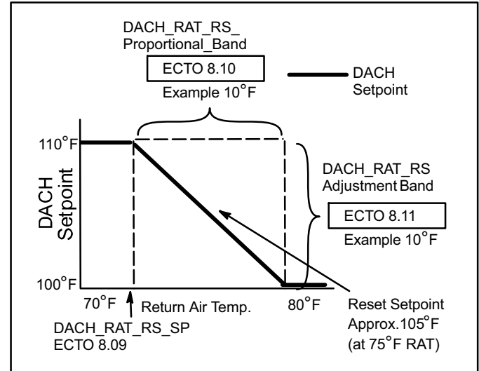
Figure 31. Return Air Reset Example
