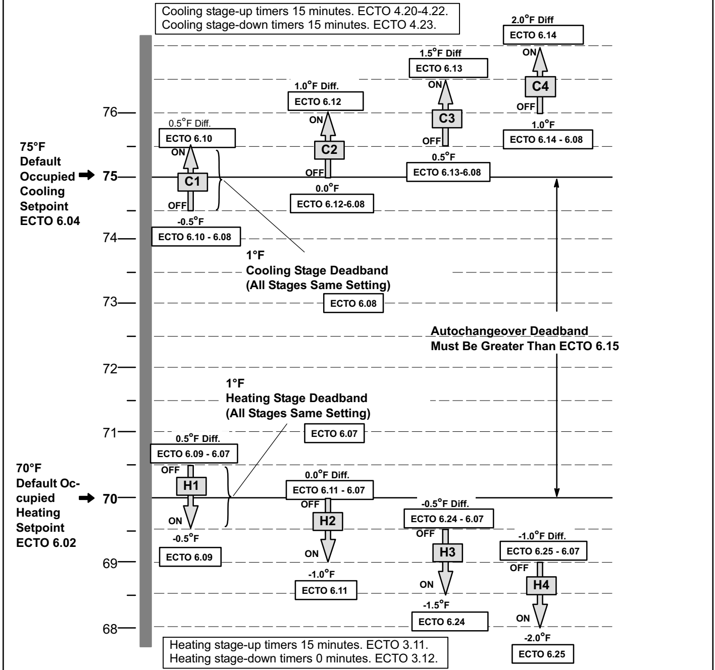
Figure 19. Zone Sensor Stages For Gas / Electric Units (Default Values Shown)
