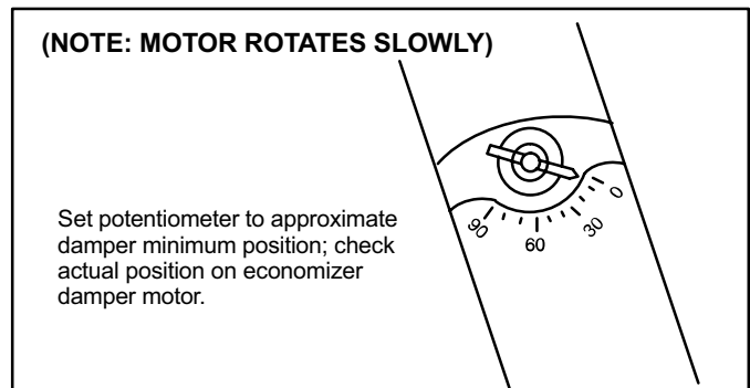
Figure 38. Economizer Damper Min. Position
