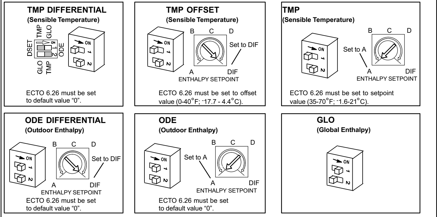
Figure 36. A56 (EM1) Free Cooling Settings
