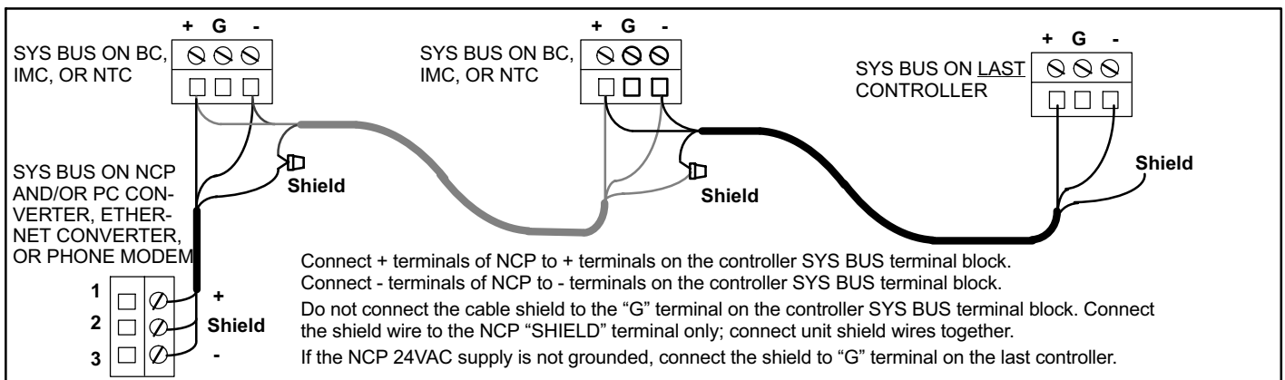
Figure 70. L Connection® Network Daisy-chain Communication Wiring
