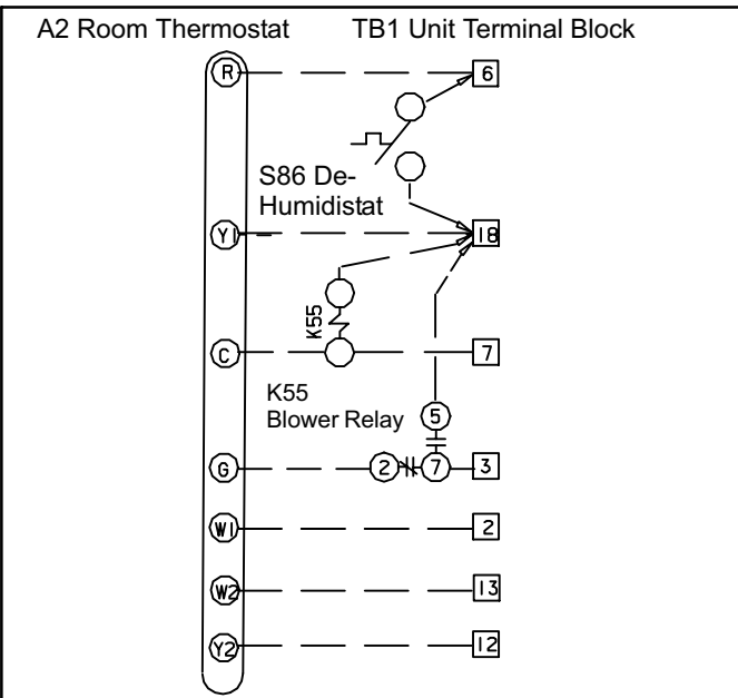
Figure 22. Supermarket Reheat Diagram (ECTO 4.24 Option 1)
