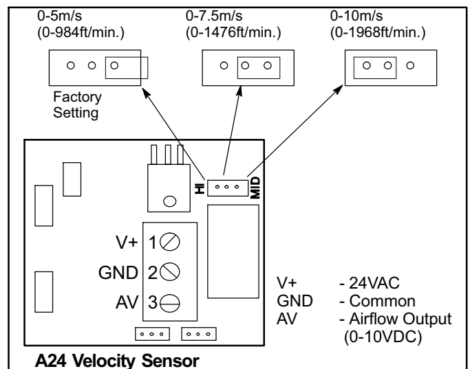
Figure 47. Velocity Sensor (A24) Range
