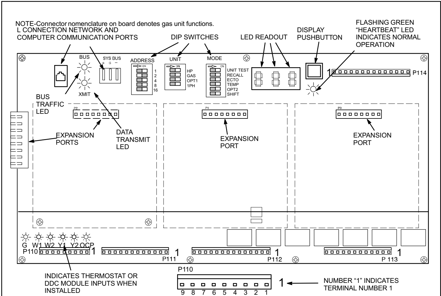
Figure 4. A55 (M1-7) Main Control Board
