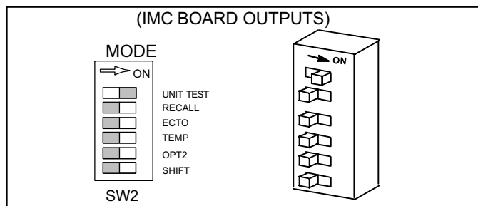
Figure 52. Mode DIP Switch Setting
