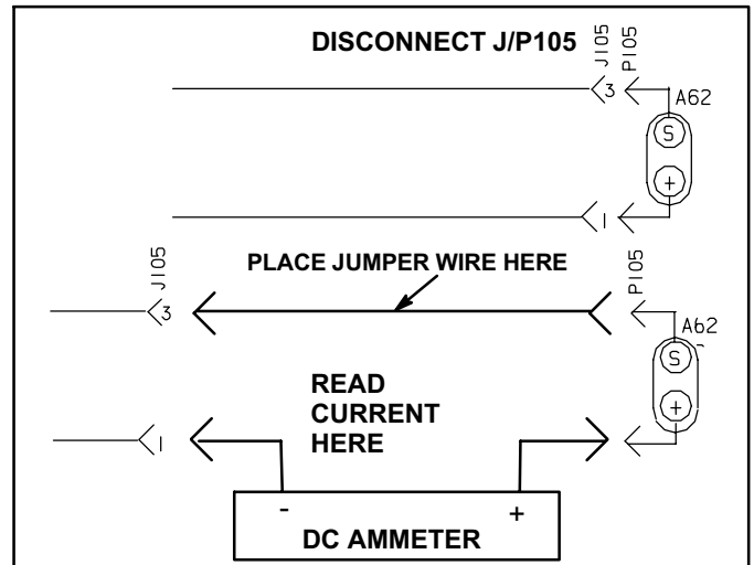
Figure 40. Measure A62 Current in Series
