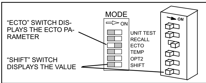
Figure 68. DIP Switch ECTO Setting
