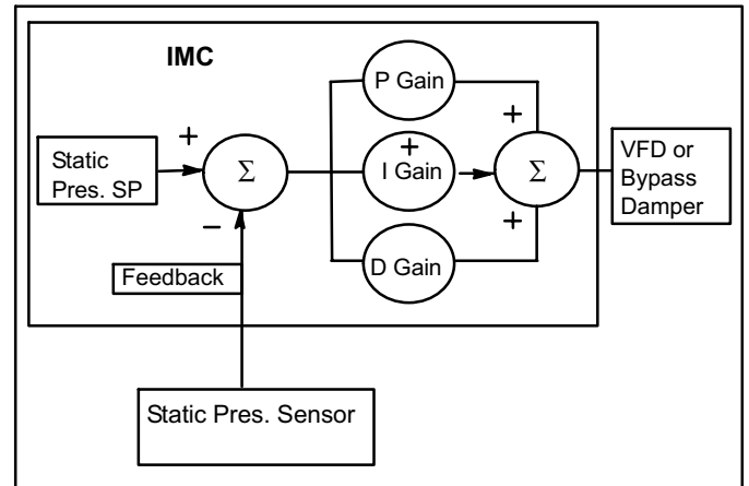
Figure 21. PID Operation Diagram For VAV/CAVB Air Delivery and Exhaust Fan Control
