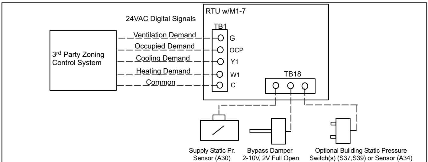
Figure 65. Field Wiring Summary for CAV Unit with Bypass Damper
