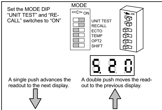
Figure 13. Read Configuration Data
