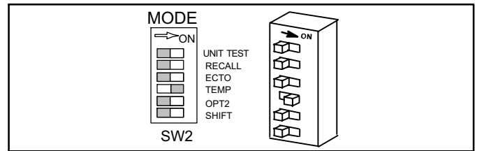
Figure 60. Display Sensor Input DIP Switch Setting
