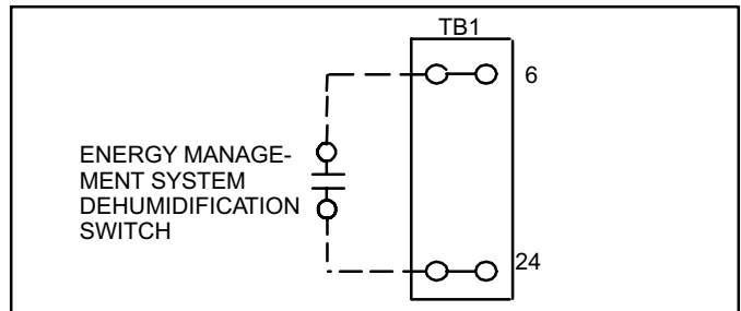
Figure 24. Humiditrol Reheat Diagram (ECTO 4.25 set to 100 for digital control)
