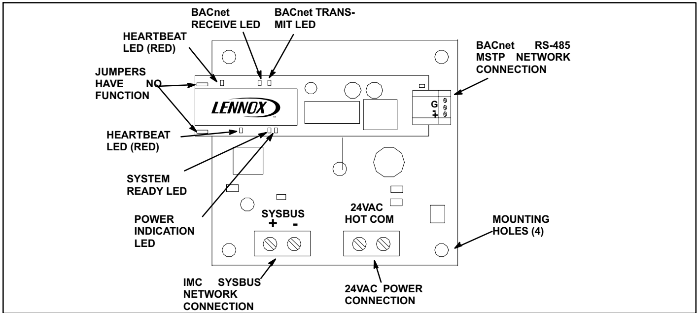
Figure 66. IMC BACnet Module (A146)
