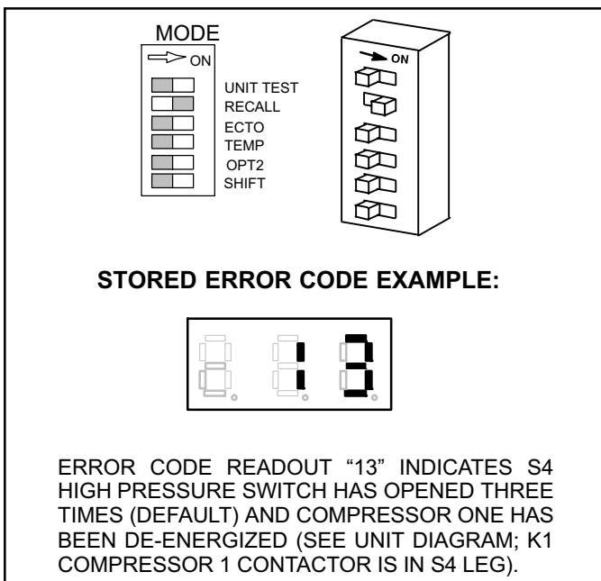
Figure 17. DIP Switch Error Code Recall Setting
