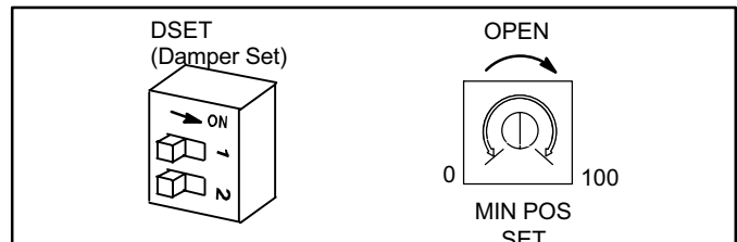
Figure 36. A56 (EM1) Free Cooling Settings
