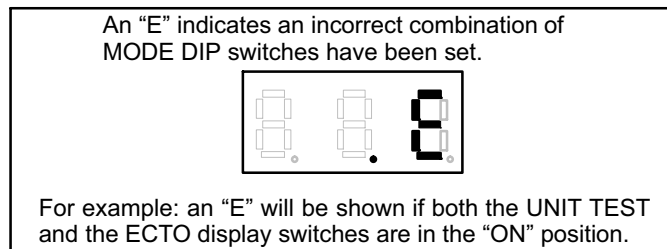
Figure 55. Incorrect Mode DIP Switch Settings Example For Digital Output —To Check Fan 3 Operation (See Figure 56):
