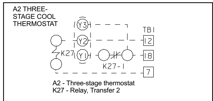
Figure 18. Three-stage Cooling (ECTO 5.04 Option 3) Wiring
