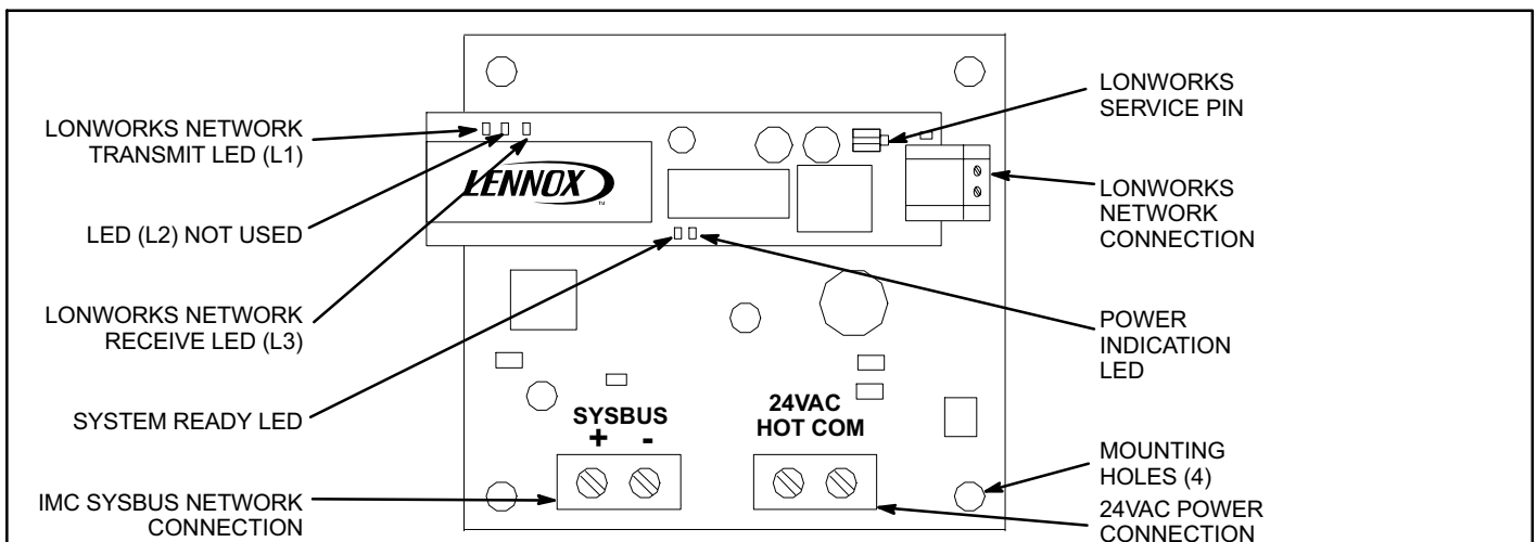
Figure 67. IMC LonTalk Module
