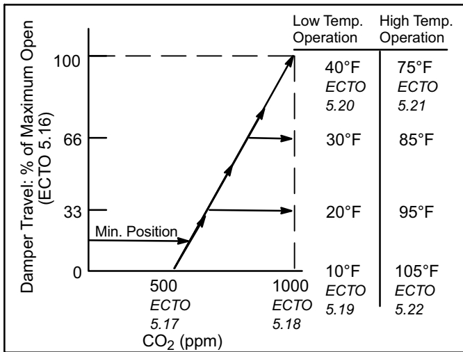
Figure 42. Default DCV Operation
