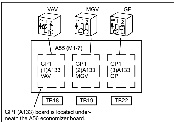
Figure 14. GP1 Board Position on IMC
