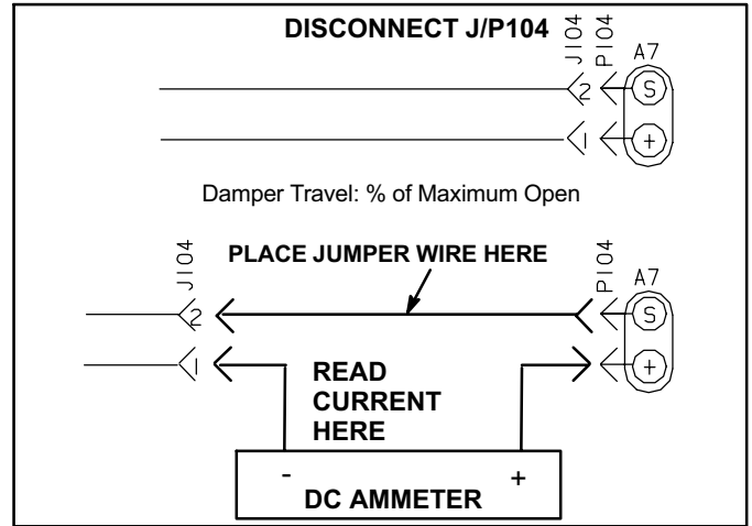
Figure 39. Measure A7 Current in Series
