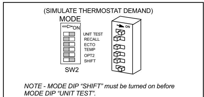
Figure 58. Mode Dip Switch Setting
