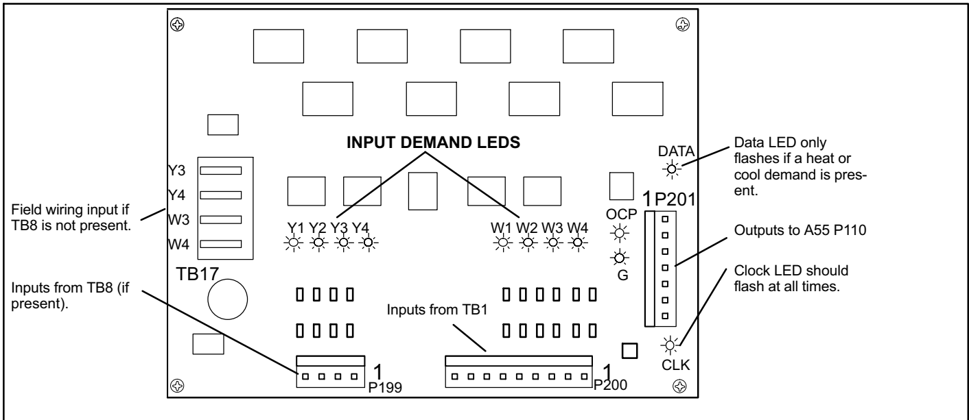
Figure 20. A138 FS1 Four Stage Board
