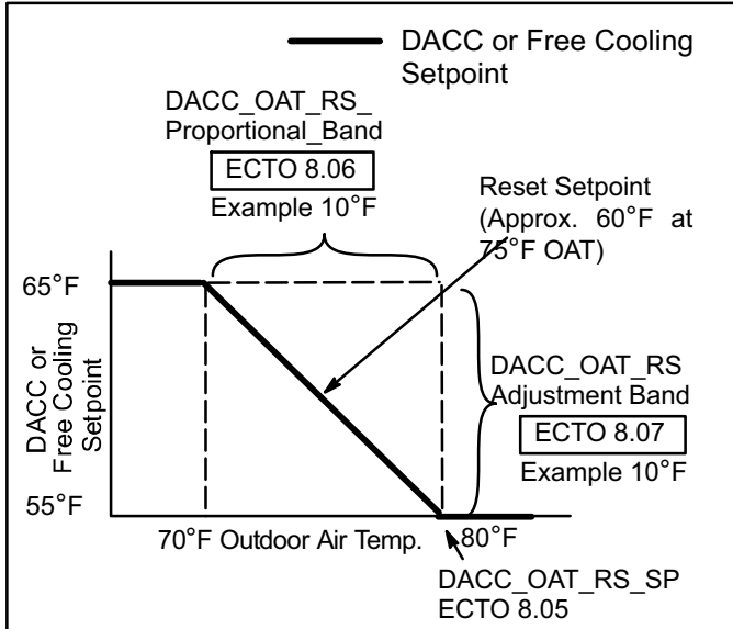
Figure 27. Outdoor Air Reset Example
