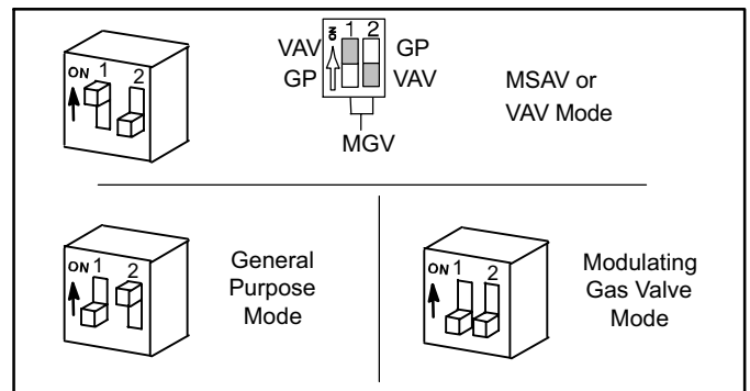
Figure 10. A133 (GP1) DIP Switch Settings
