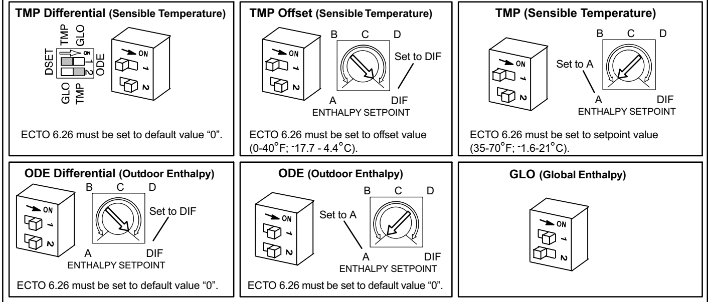
Figure 11. A56 (EM1) Free Cooling Settings
