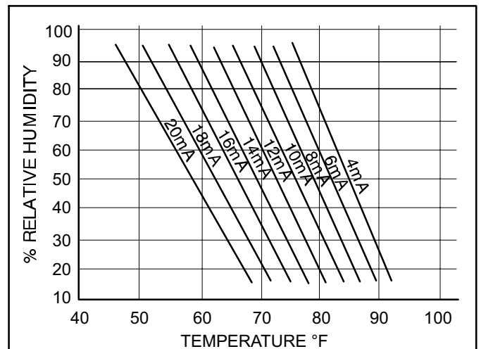
Figure 41. Enthalpy Sensor Output Current Honeywell C7400
