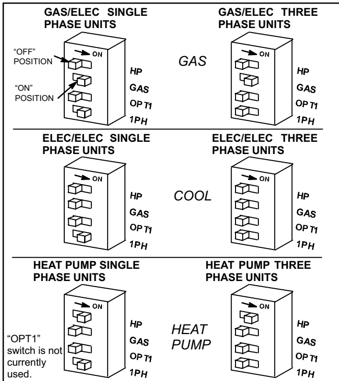
Figure 7. Unit DIP Switch Settings (A55)
