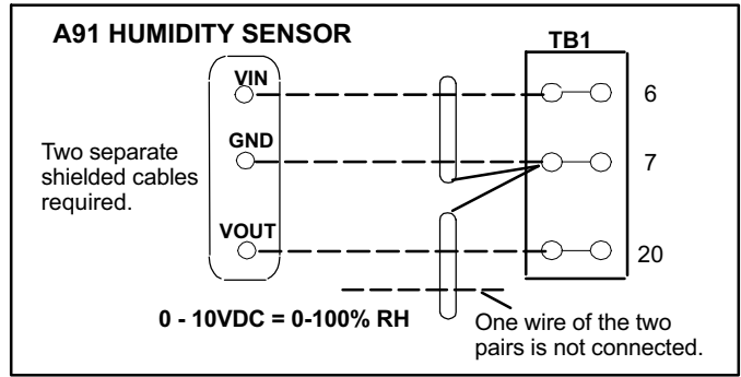
Figure 23. Reheat Sensor Diagram
