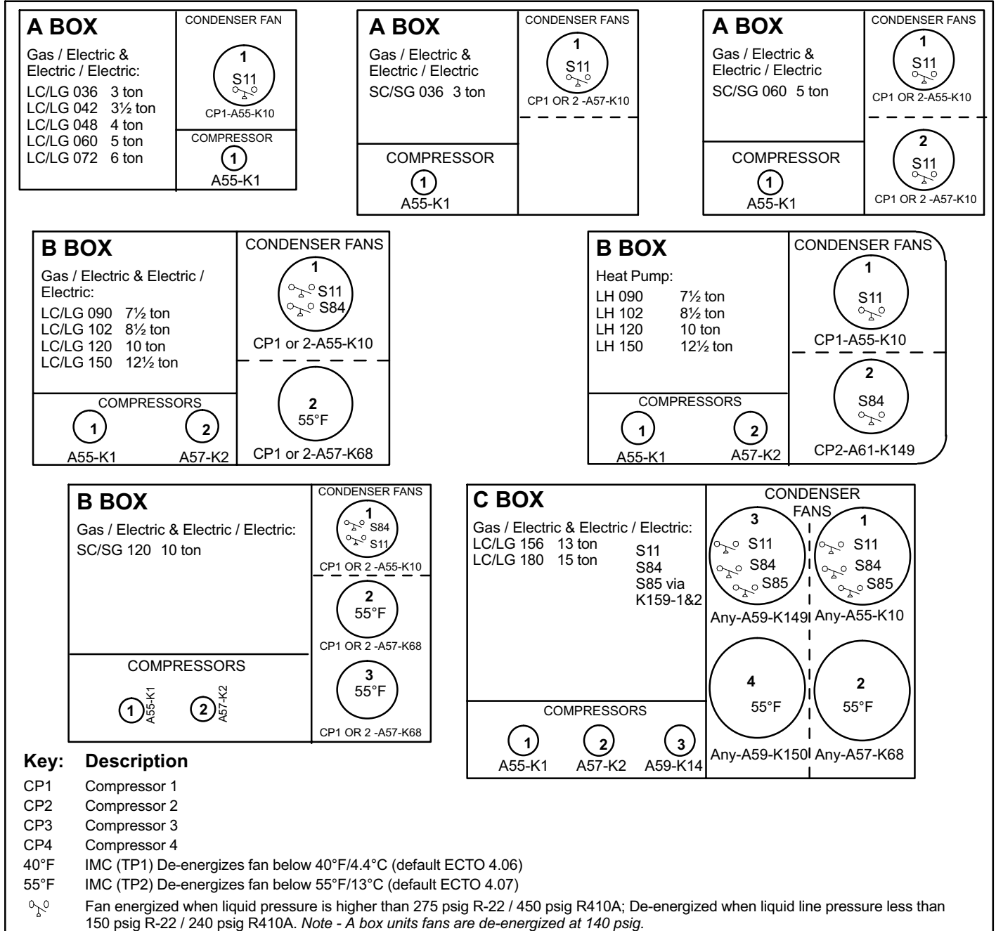
Figure 33. Compressor and Fan Operation (top view of unit not to scale)
