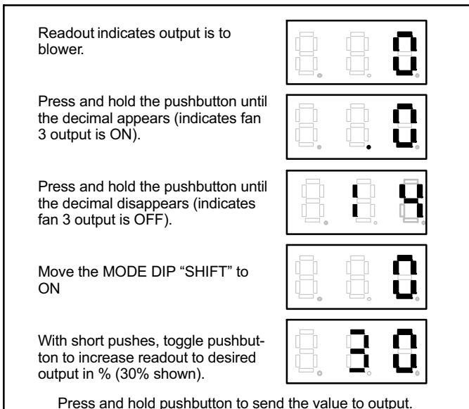
Figure 57. Energize Variable Speed Blower
