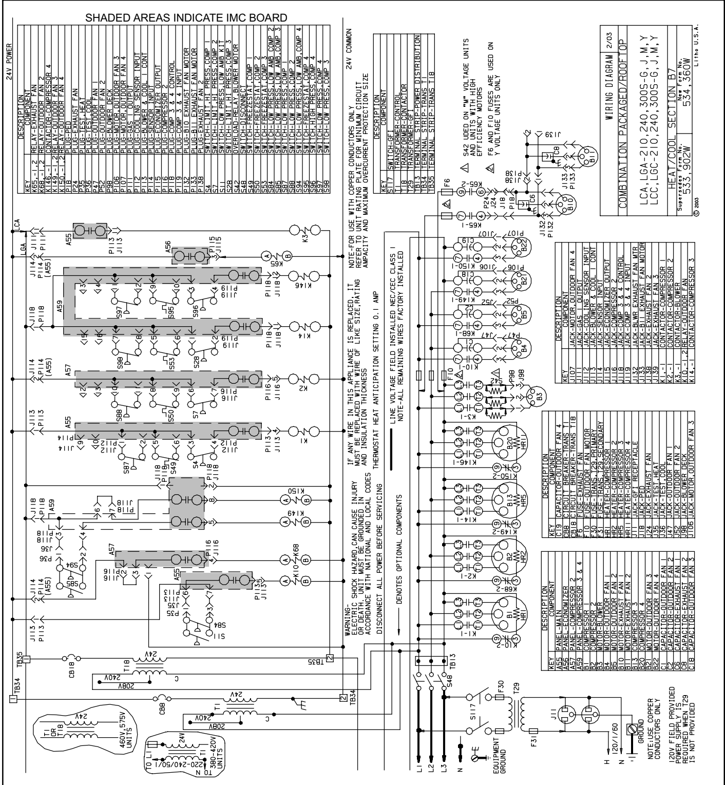
Figure 71. Typical 17-1/2 & 20 Ton Wiring Diagram
