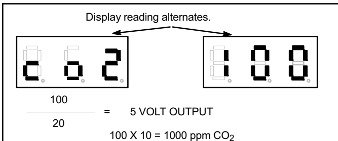
Figure 62. IAQ Sensor Output Voltage
