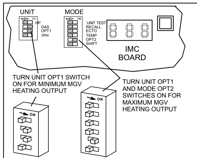
Figure 32. Initiate Maximum & Minimum MGV
