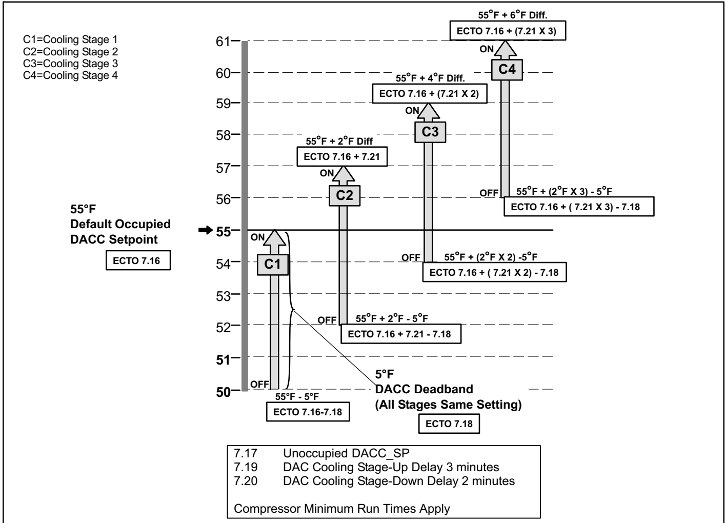
Figure 26. Discharge Air Control Cooling (DACC) Stages - Default Values Shown
