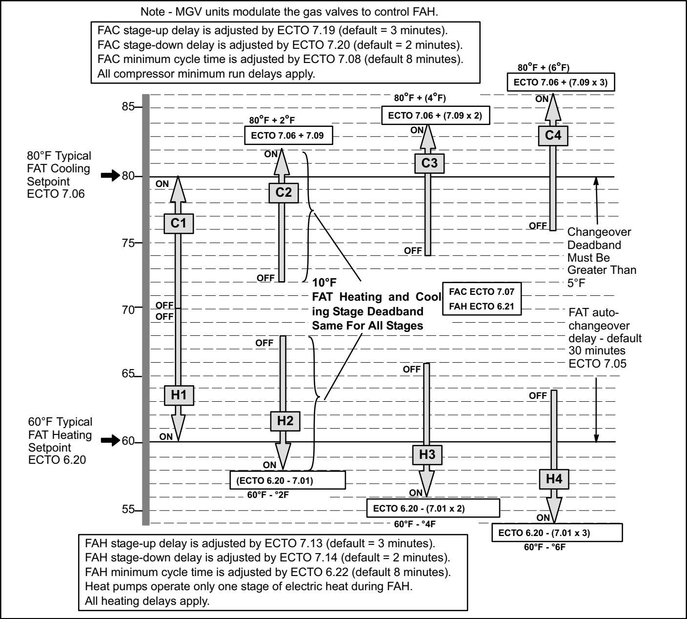
Figure 25. Fresh Air Tempering (FAT) Stages - Default Values Shown
