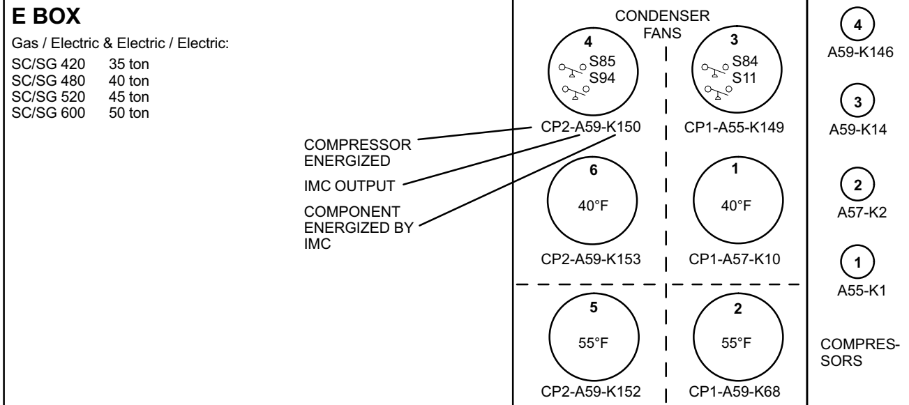
Figure 34. Compressor and Fan Operation (top view of unit not to scale)
