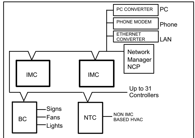
Figure 69. L Connection Network
