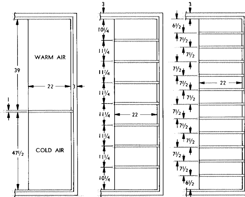
SUPPLY AIR CONNECTIONS FOR DOUBLE DUCT APPLICATIONS
