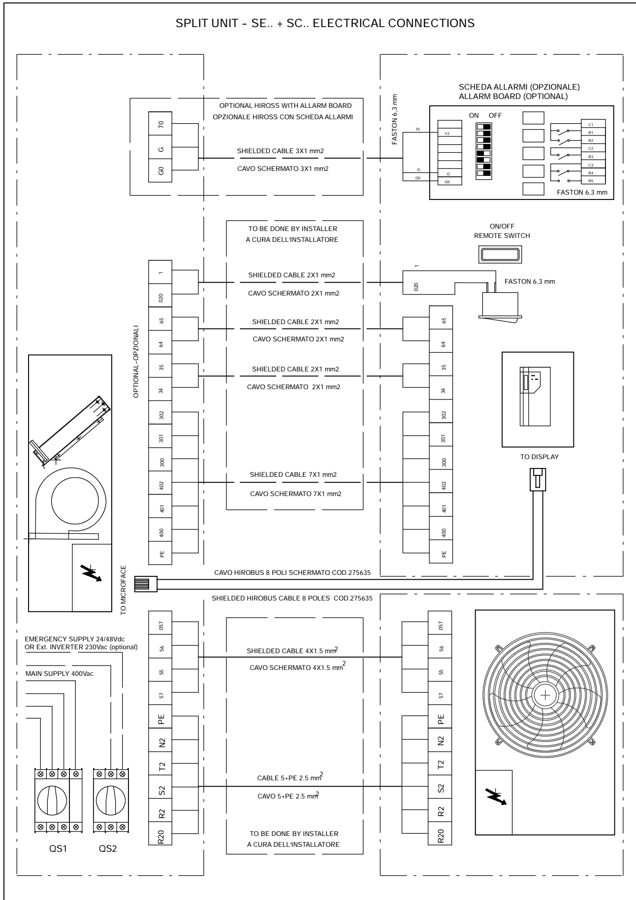
Fig.6a – Electrical diagram SE+ SC 08–10–13–14 / Schema elettrico SE+ SC 08–10–13–14
