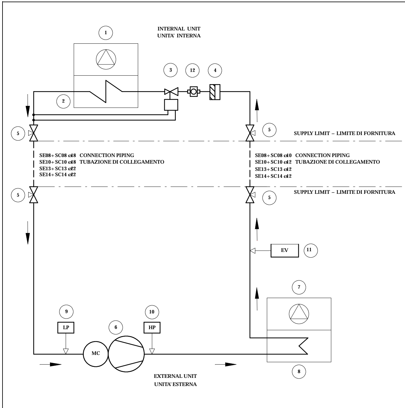
Fig. 12 – Refrigeration circuit / Schema frigorifero SE+ SC 08–10–13–14
