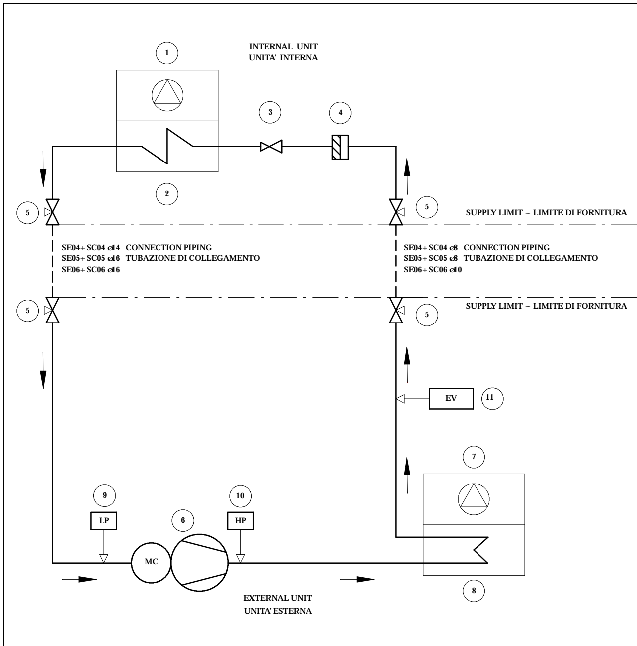
Fig. 11 – Refrigeration circuit / Schema frigorifero SE+ SC 04–05–06
