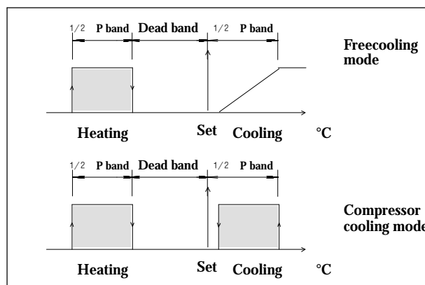
Fig. K – Operation of compressor, electric heaters and opening of the Freecooling damper
