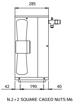
SIDE VIEW / VISTA LATERALE
