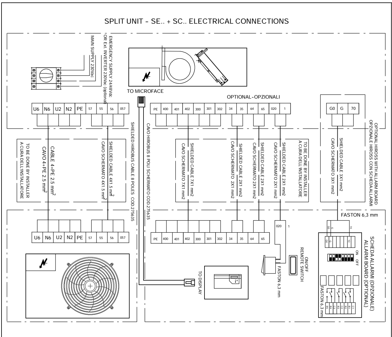
Fig. 7 – Electrical diagram SE+ SC 04–05–06 / Schema elettrico SE+ SC 04–05–06
