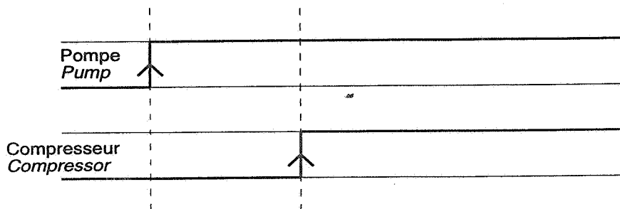
Retard entre pompe et compresseur Time-delay between pump and compressor
