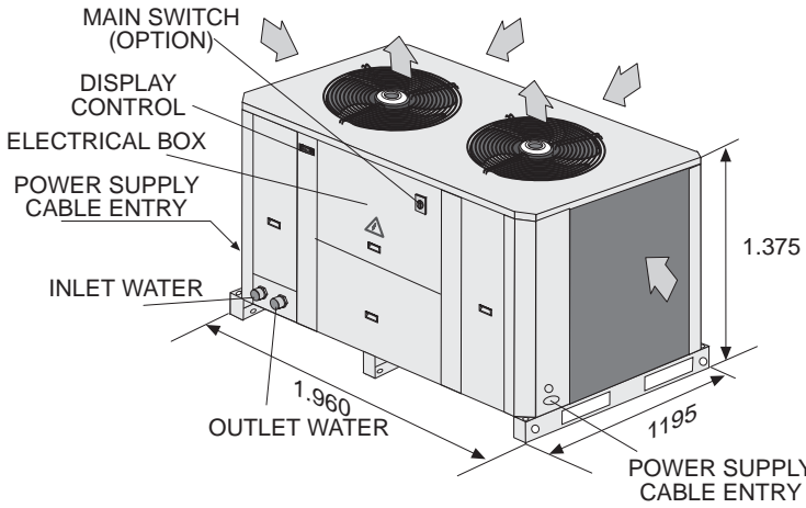
EAC/EAR 0472S-0552S-0672S-0812S
