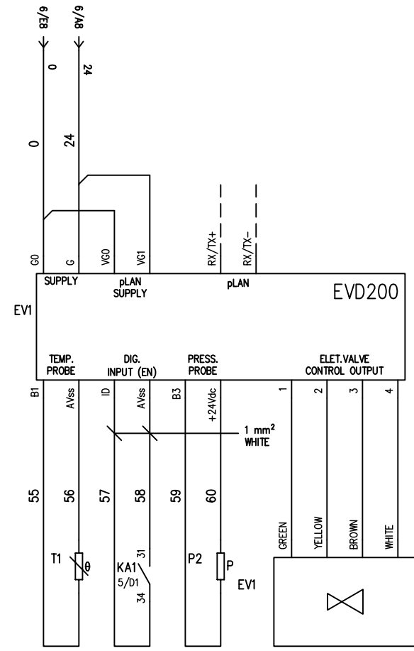
ELECTRONIC EXPANSION VALVE OPTION
