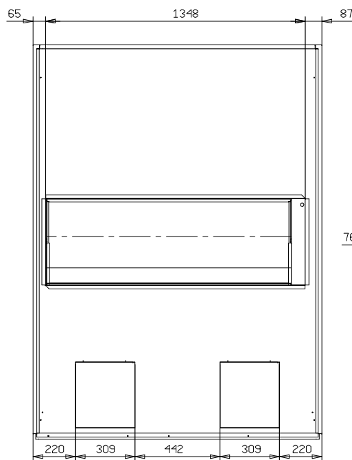
HTU 220-250 REAR VIEW
