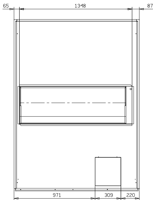
HTU 180-200 REAR VIEW
