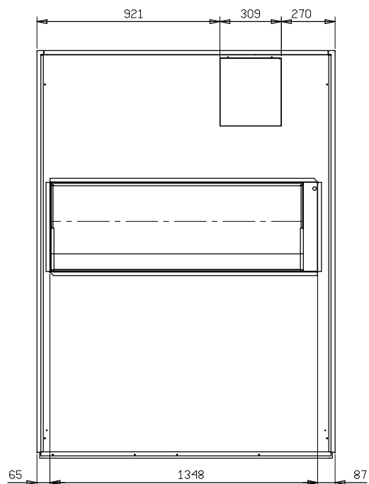
HTD 180-200 REAR VIEW
