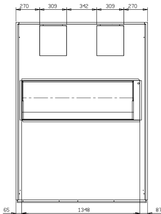
HTD 220-250 REAR VIEW
