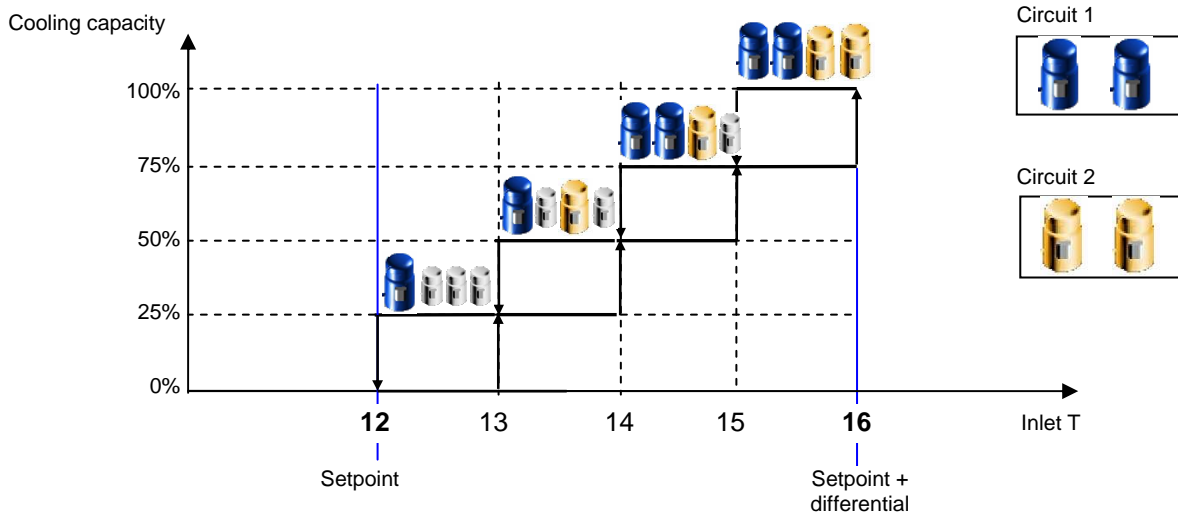
Figure 7: Balanced Rotation
