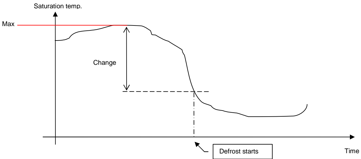
Figure 19: Change-Based Logic
