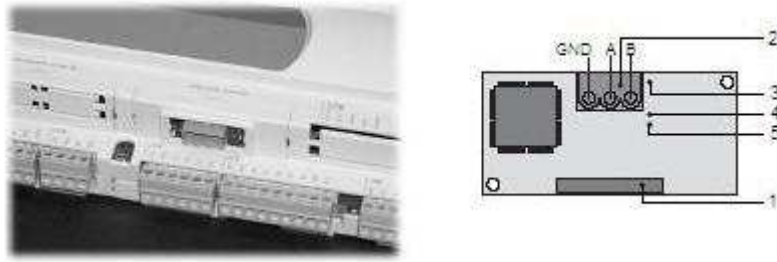
Figure 31: LON card
