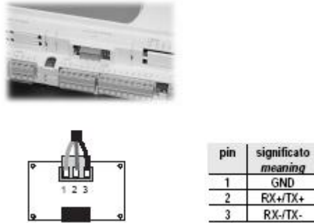
Figure 30: RS485 Serial Card
