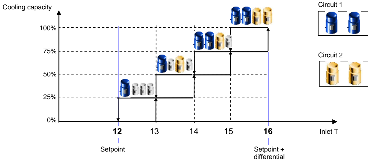
Figure 7: Balanced Rotation
