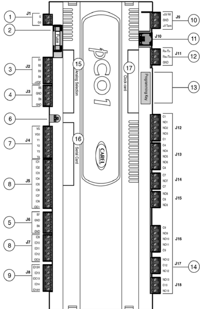
Figure 15: Layout
