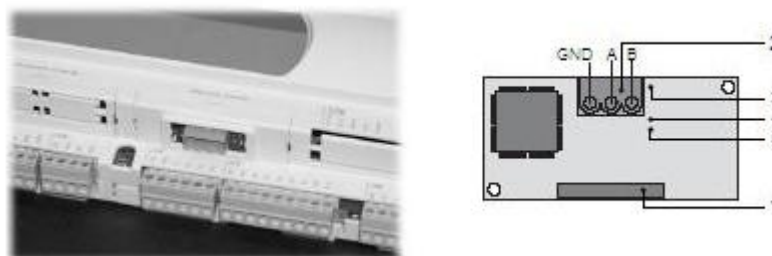
Figure 31: LON card
