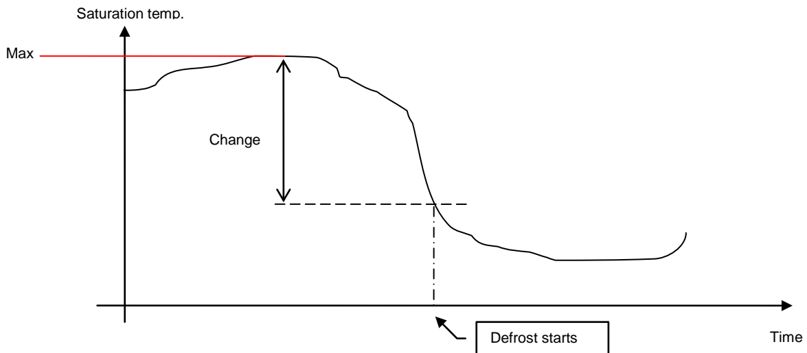
Figure 19: Change-Based Logic
